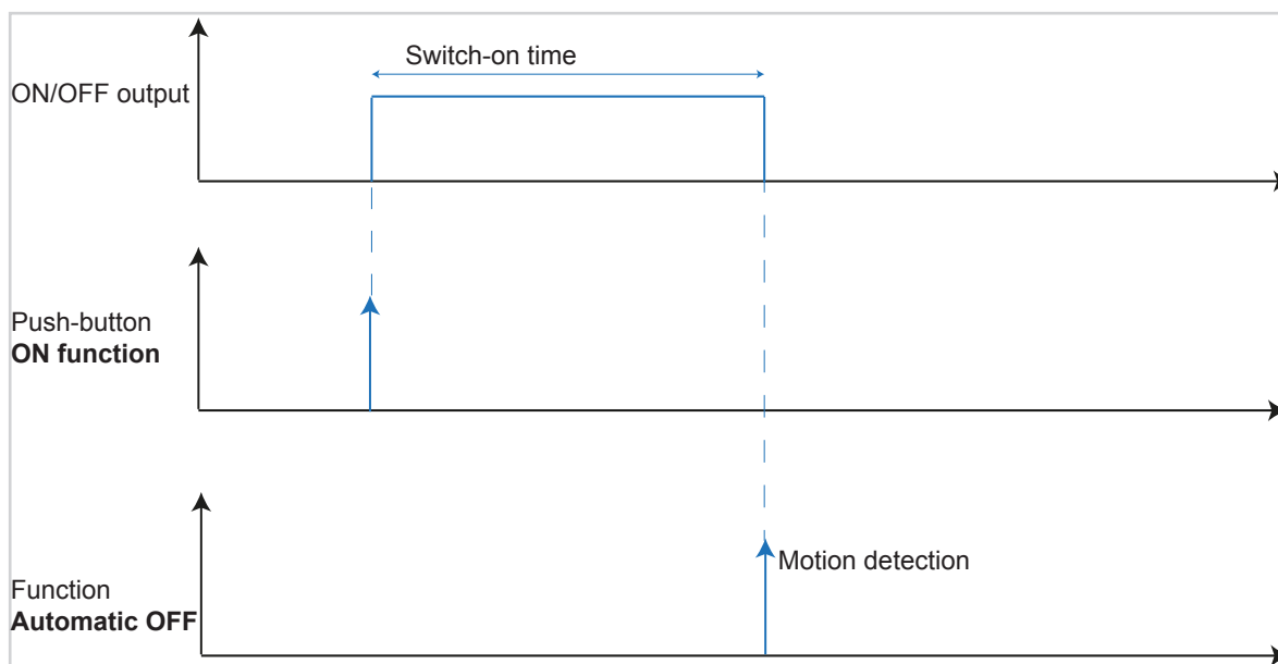
Figure 15: Signal-time diagram for Automatic OFF
