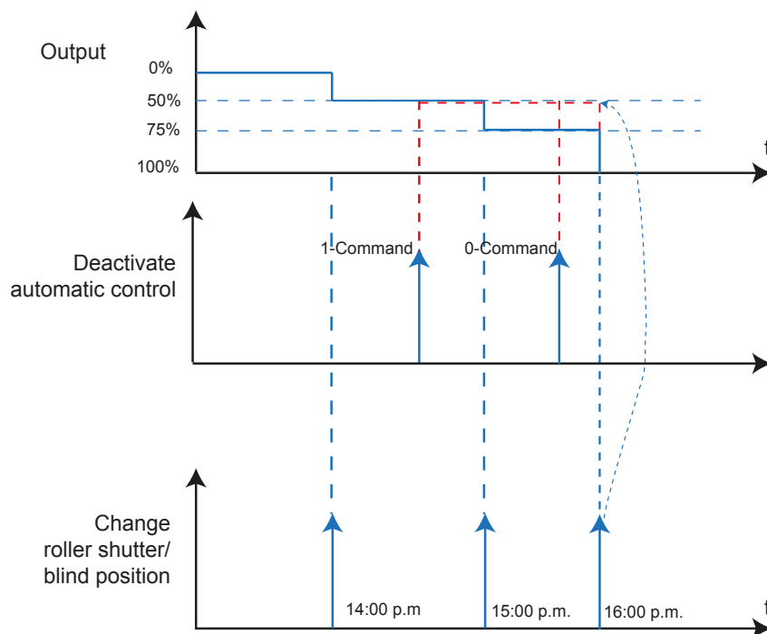
Figure 53: Signal-time diagram for Automatic control deactivation
