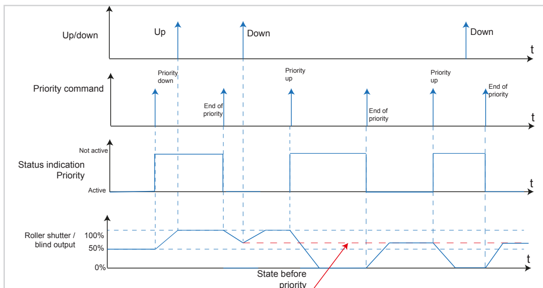
Figure 51: Signal-time diagram for Priority roller shutter/blind
